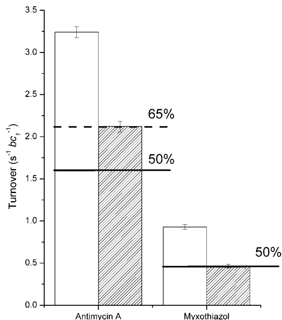
FIGURE 2: The antimycin A- and myxothiazol-resistant reduction of cyt c is partially inhibited by Mn-SOD. This figure shows the effect of the addition of excess Mn-SOD on the myxothiazol- and antimycin A-resistant reduction of cyt c . The results are expressed in moles of cyt c reduced per second per mole of cyt bc 1 . Experimental conditions were the same as in Figure 1. The bar graph shown is an average of three repeats. Key: empty bars, no additions; hatched bars, +300 units of Mn-SOD.
