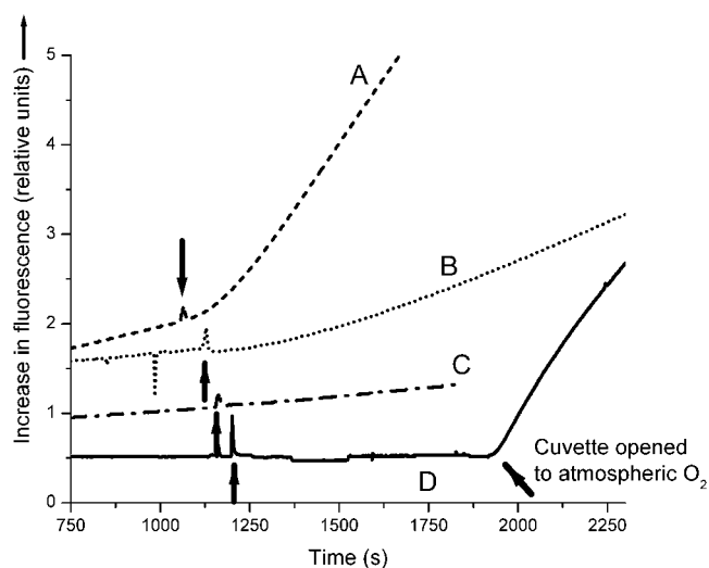
FIGURE 3: Myxothiazol and antimycin A but not stigmatellin induce H 2 O 2 /O 2 - production in the isolated cyt bc 1 complex. The experiment was carried out in bc 1 reaction buffer (pH 6.90) at room temperature. The buffer also contained 400 μM Amplex Red, 10 units/mL horseradish peroxidase, and 300 units of Mn-SOD. Substrates (50 μM decylubiquinol, 50 μM cyt c ) were added to start the experiment. A background trace was obtained, after which 42 nM cyt bc 1 complex was added to the reaction mixture (indicated by the dark gray arrow). Trace A contains substrates, Mn-SOD, and 20 μM antimycin A. Trace B contains the same as in (A) + 20 μM myxothiazol. Trace C contains the same as in (A) + 5 μM stigmatellin. Trace D contains the same as in (A) but conducted under anaerobic conditions. The light gray arrow at the end of the trace indicates where the argon flow was stopped, the anaerobic cuvette opened to the atmosphere, and air blown through the system.
